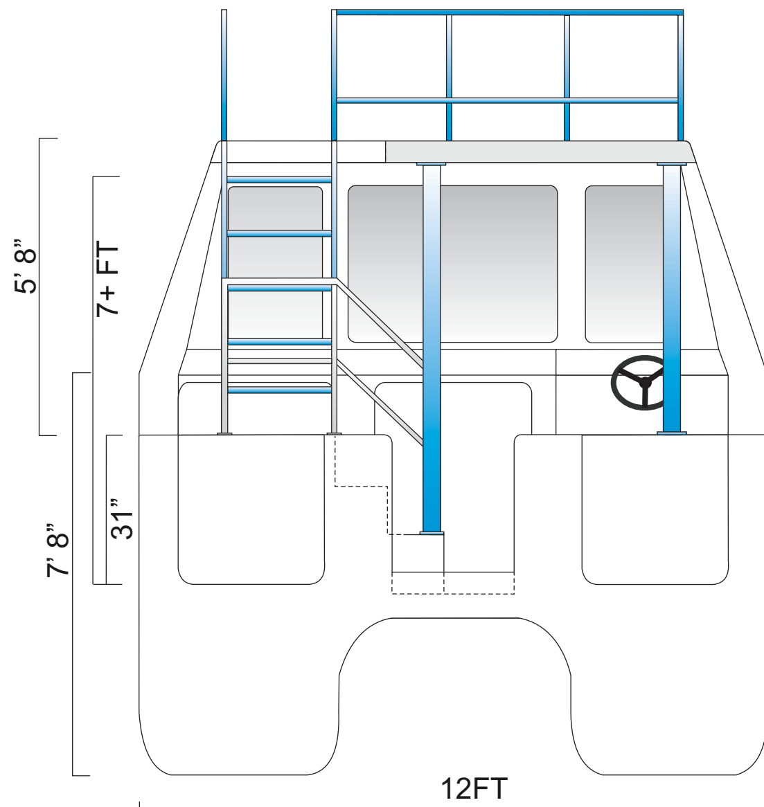
REAR PLAN
