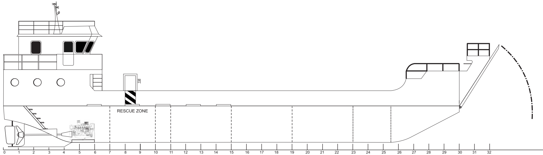
PROFILE
